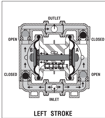
LEFT STROKE FIGURE 2 When the pressurized diaphragm, diaphragm A, reaches the limit of its discharge stroke, the air valve redirects pressurized air to the back side of diaphragm B. The pressurized air forces diaphragm B away from the center block while pulling diaphragm A to the center block. Diaphragm B is now on its discharge stroke. Diaphragm B forces the inlet valve ball onto its seat due to the hydraulic forces developed in the liquid chamber and manifold of the pump. These same hydraulic forces lift the discharge valve ball off its seat, while the opposite discharge valve ball is forced onto its seat, forcing fluid to flow through the pump discharge. The movement of diaphragm A toward the center block of the pump creates a vacuum within liquid chamber A. Atmospheric pressure forces fluid into the inlet manifold of the pump. The inlet valve ball is forced off its seat allowing the fluid being pumped to fill the liquid chamber.
