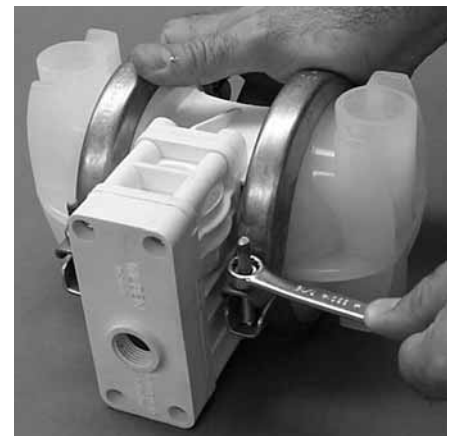
Step 8. Figure 8 Use a 11 mm (7/16") wrench to remove one set of clamp bands that secure one liquid chamber to the one-piece center section.
