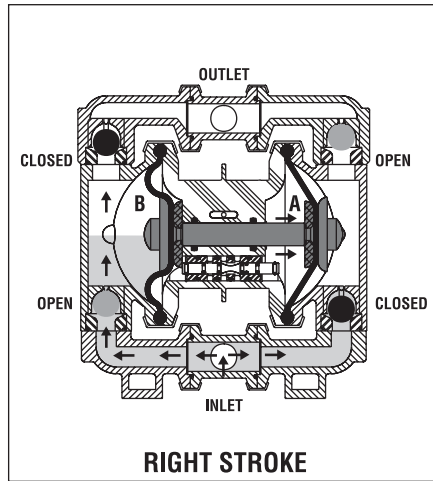
RIGHT STROKE FIGURE 1 The air valve directs pressurized air to the back side of diaphragm A. The compressed air is applied directly to the liquid column separated by elastomeric diaphragms. The diaphragm acts as a separation membrane between the compressed air and liquid, balancing the load and removing mechanical stress from the diaphragm. The compressed air moves the diaphragm away from the center block of the pump. The opposite diaphragm is pulled in by the shaft connected to the pressurized diaphragm. Diaphragm B is on its suction stroke; air behind the diaphragm has been forced out to the atmosphere through the exhaust port of the pump. The movement of diaphragm B toward the center block of the pump creates a vacuum within chamber B. Atmospheric pressure forces fluid into the inlet manifold forcing the inlet valve ball off its seat. Liquid is free to move past the inlet valve ball and fill the liquid chamber (see shaded area).
