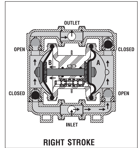
RIGHT STROKE FIGURE 3 At completion of the stroke, the air valve again redirects air to the back side of diaphragm A, which starts diaphragm B on its exhaust stroke. As the pump reaches its original starting point, each diaphragm has gone through one exhaust and one discharge stroke. This constitutes one complete pumping cycle. The pump may take several cycles to completely prime depending on the conditions of the application.
